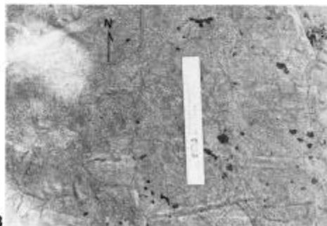
Plate 1. Sketch map of a small outcrop in Skelton Creek with photographs A, B, and C which show faults with strike separation. Locations of the photographs are shown on the sketch map.
