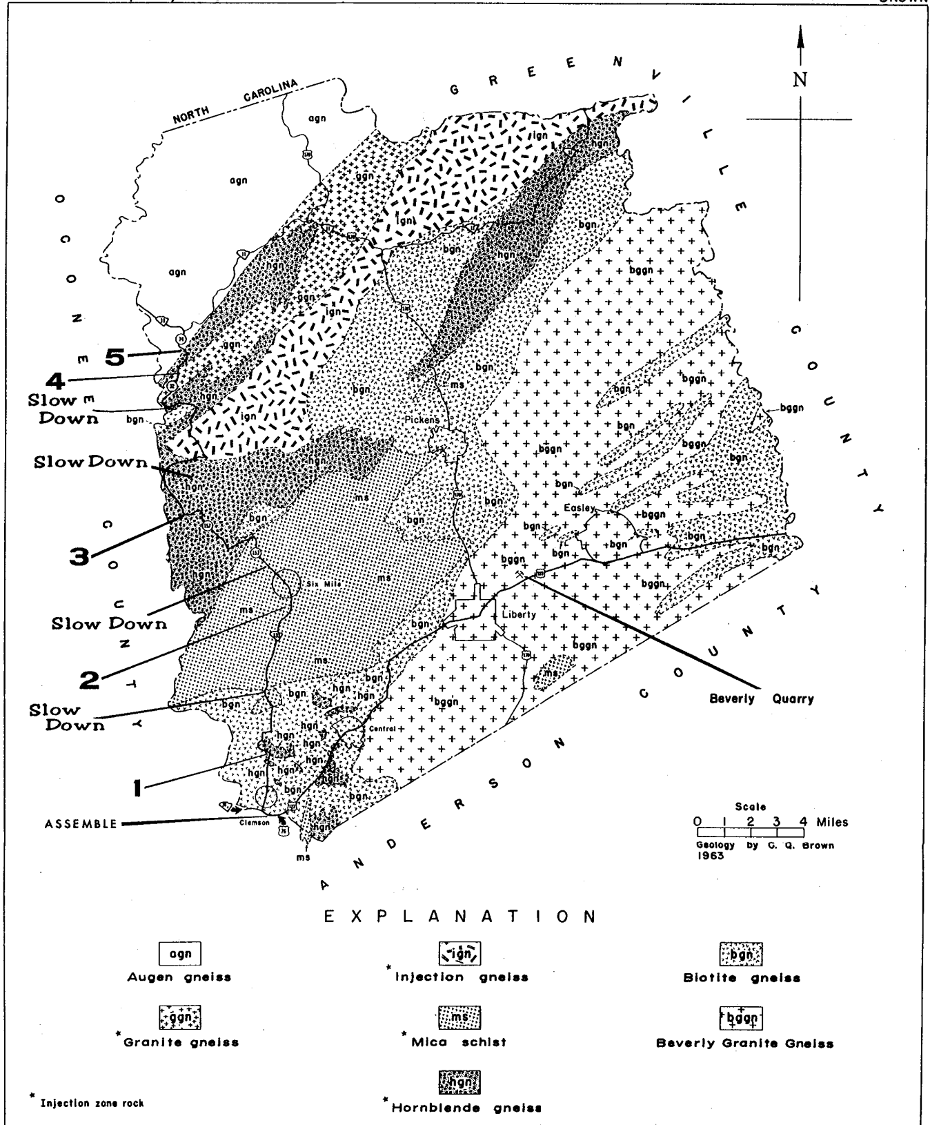
Figure 1. Generalized geologic map of Pickens County, South Carolina
