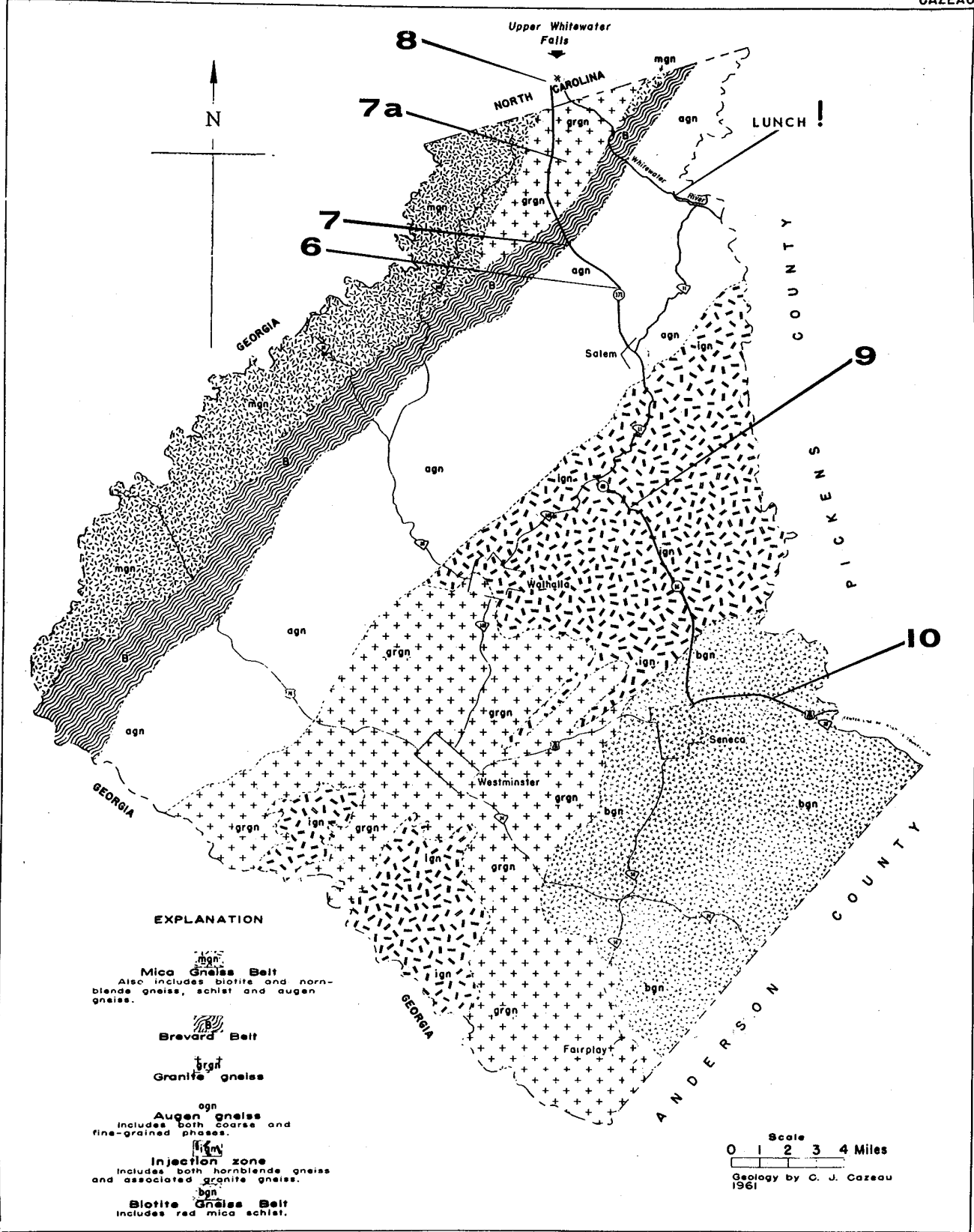
Figure 2. Generalized geologic map of Oconee County, South Carolina.
